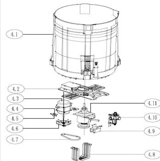
c: Outer Tub Subassembly
