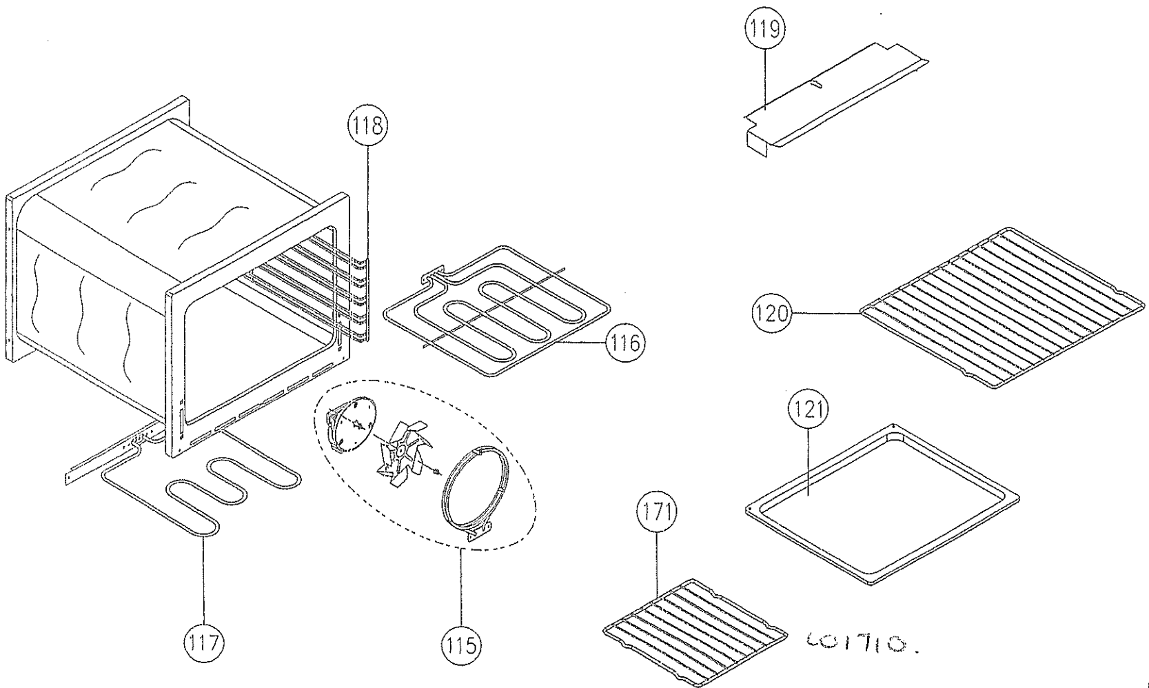
Drawing 05 - Multifunction oven 8 functions
