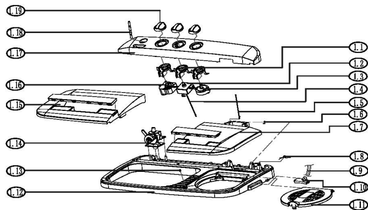
1:Top Cover Subassembly
