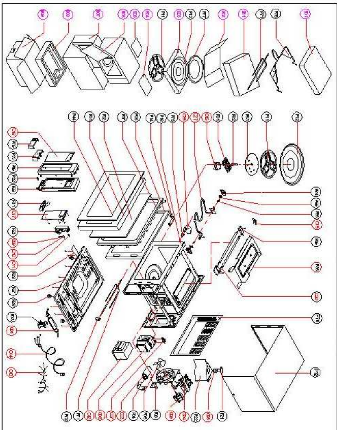
WD300ASP28D41-5S Microwave Oven Explode Drawing (3)
