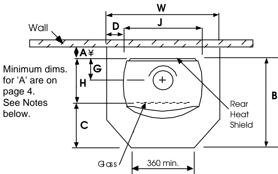
MINIMUM HEARTH EXTENSIONS (mm) WHEN THE REAR HEAT SHIELD IS FITTED
