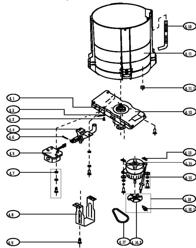
c: Outer Tub Subassembly
