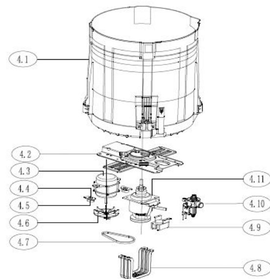
c: Outer Tub Subassembly
