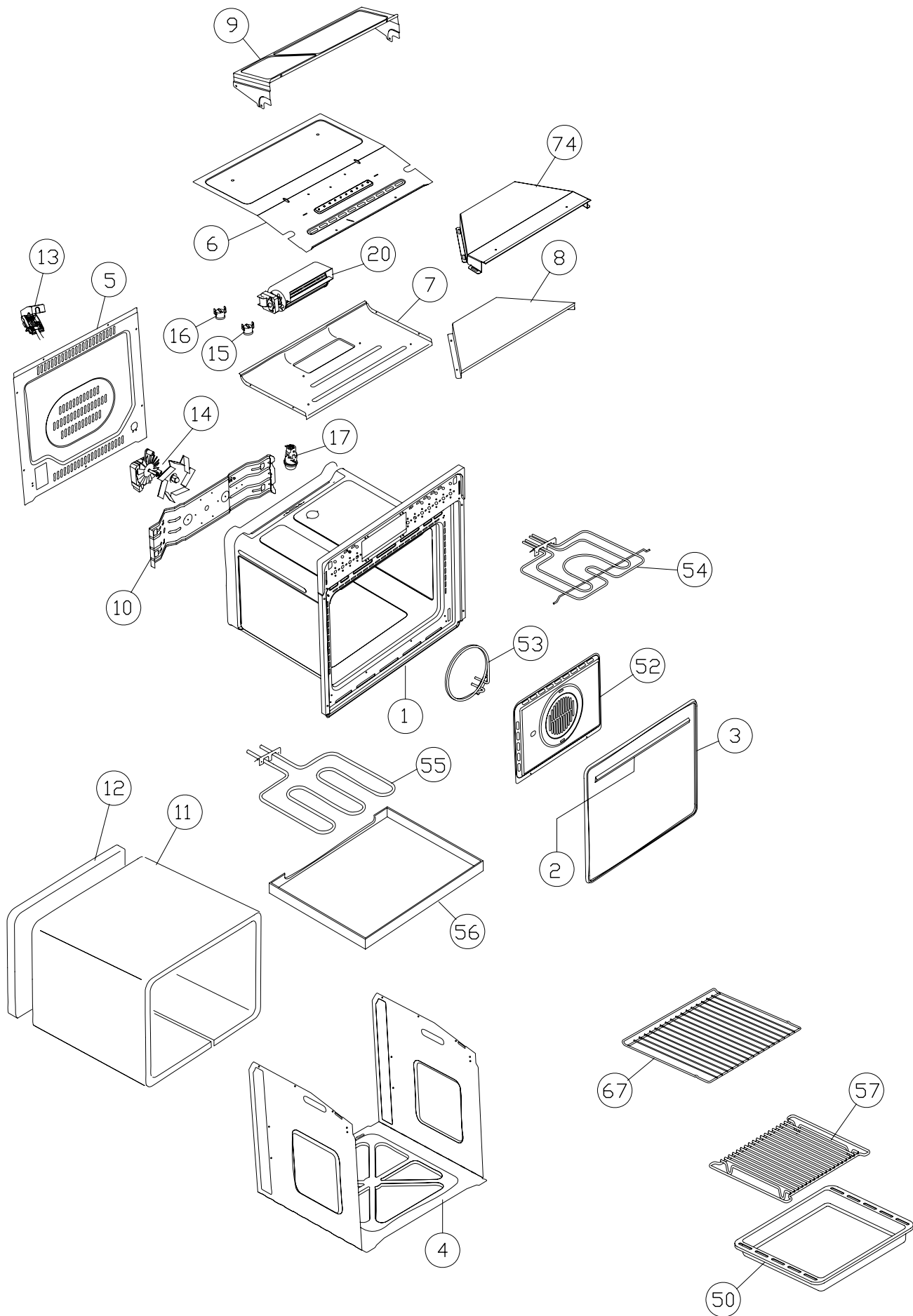
REFLEX1 - FM80E
