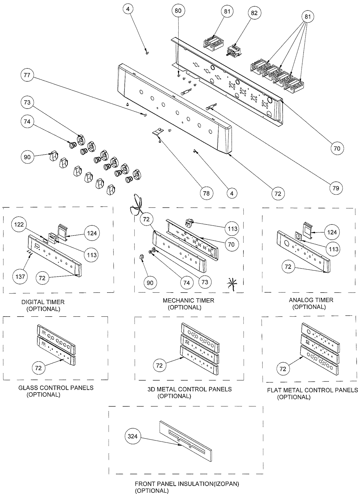
EXPLODED VIEW - CONTROL PANEL ASSEMBLY
