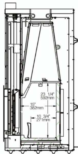
Combustion chamber
