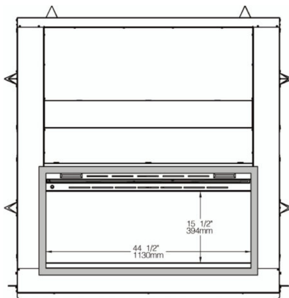
Door opening black straight narrow trim
