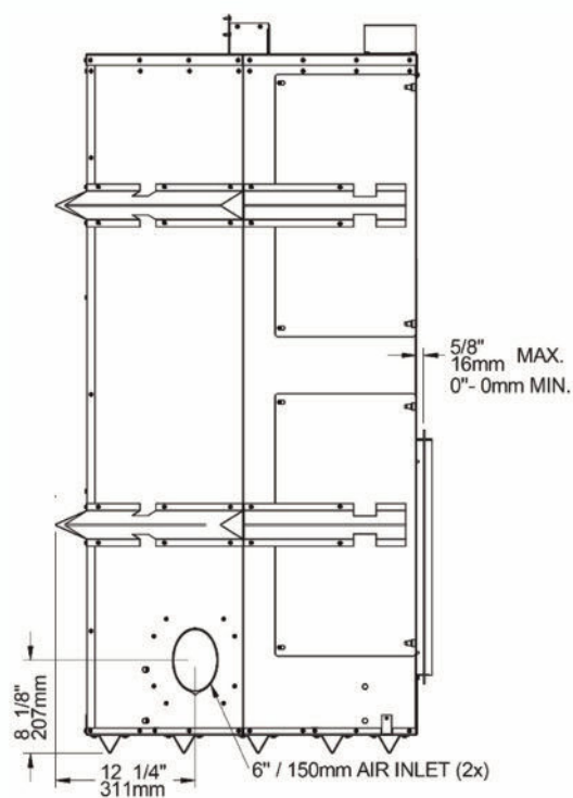
Left side black straight masonry trim
