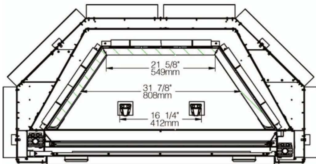
Combustion chamber
