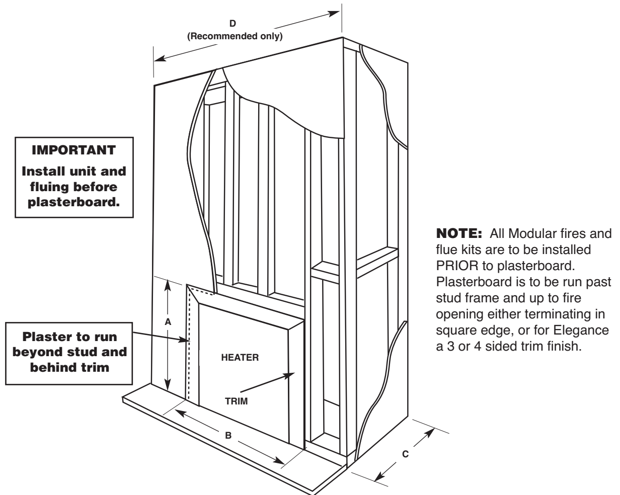
Frameout Dimensions (in mm)
