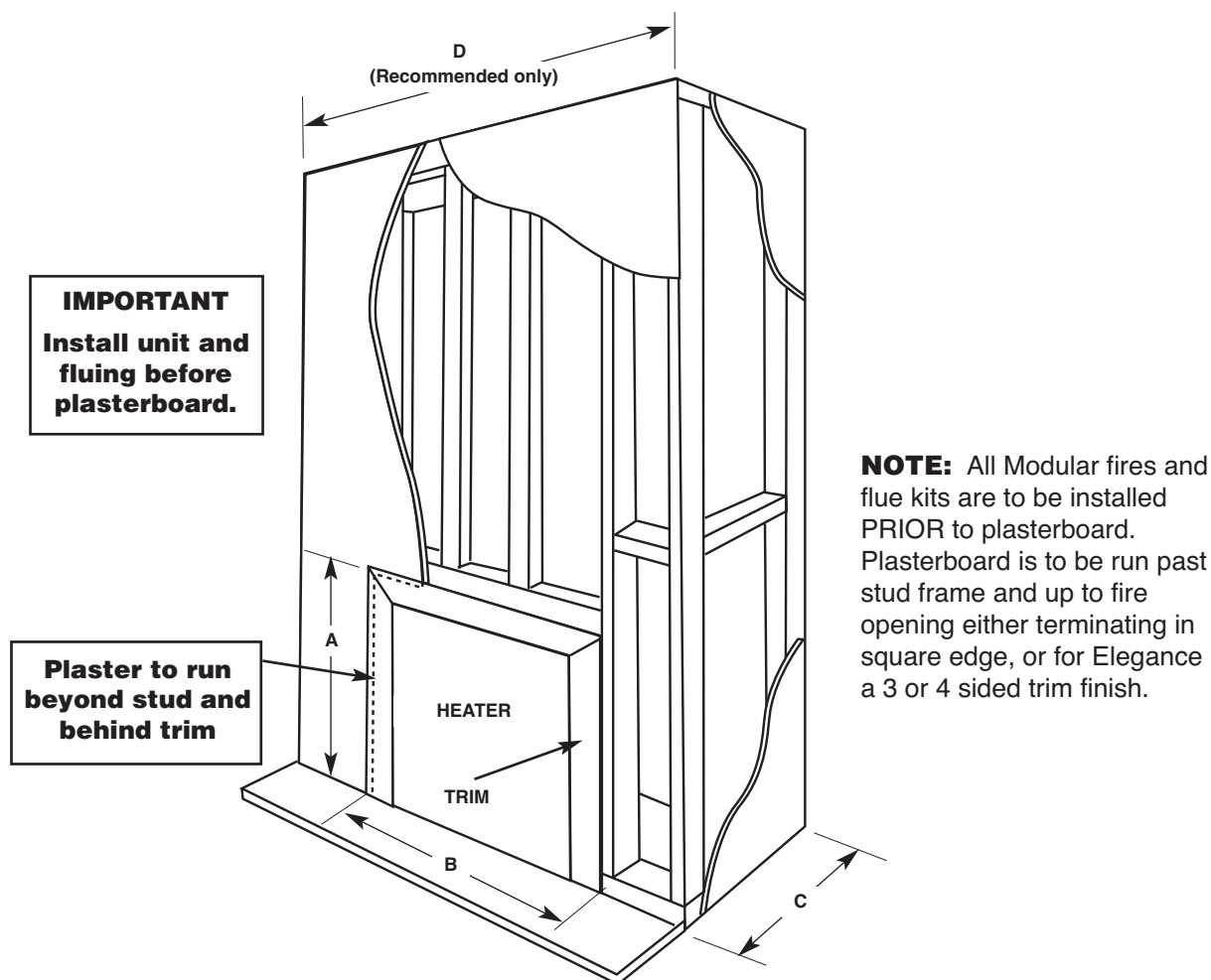
Frameout Dimensions (in mm)
