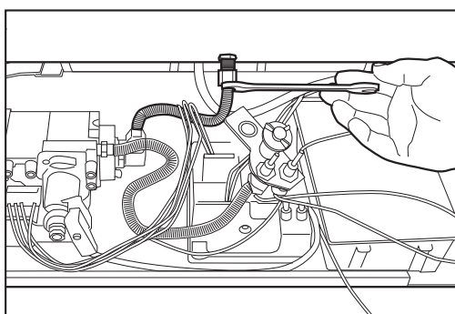
Figure (20) Undo the flexi tube from the bulk head.
